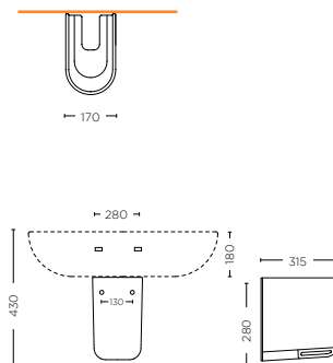
SEMICOLONNA HALF PEDESTAL SDBD.PD.10.02
