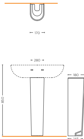
COLONNA PEDESTAL SDBD.PD.10.01
