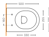
VASO FILO MURO 50R BACK TO WALL WC 50R SMMX.20.F01R
