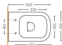
VASO SOSPEO 50Q WALL HUNG WC 50Q SMMX.20.W01Q
