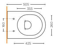
VASO SOSPEO 50R WALL HUNG WC 50R SMMX.20.W01R
