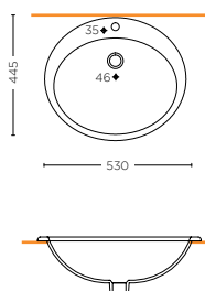
LAVABO OVER DA INCASSO 53 cm OVER COUNTER WASHBASIN 53 cm
