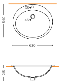
LAVABO DA INCASSO OVER 63 cm OVER COUNTER WASHBASIN 63 cm
