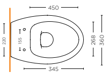
VASO FILO MURO BACK TO WALL WC SDBD.20.F01
