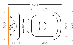
VASO MONOBLOCCO CON CASSETTA 66Q CLOSE COUPLED WC WITH CISTERN 66Q MMX.20.C02Q / SMMX.28.02
