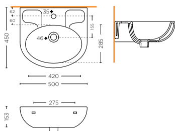
LAVABO 50 cm WASHBASIN 50 cm WITH SOAP DISH SDBD.10.05
