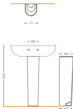
COLONNA PEDESTAL SECO.PD.10.01
