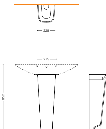
COLONNA PEDESTAL SCLB.PD.10.01
