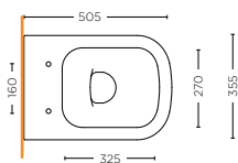
VASO FILO MURO 50Q BACK TO WALL WC 50Q SMMX.20.F01Q
