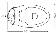
VASO MONOBLOCCO CON CASSETTA SCARICO A PARETE CLOSE COUPLED WC WITH CISTERN P-TRAP SDBD.20.C11 / SDBD.28.10
