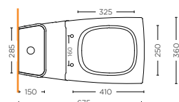
VASO ONE PIECE ONE PIECE WATER CLOSET SMAJ.20.OP01
