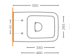
VASO FILO MURO BACK TO WALL WC SCLB.20.F01
