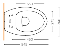
VASO SOSPESO WALL HUNG WC SDBD.20.W01
