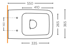
VASO SOSPESO WALL HUNG WC SCLB.20.W01
